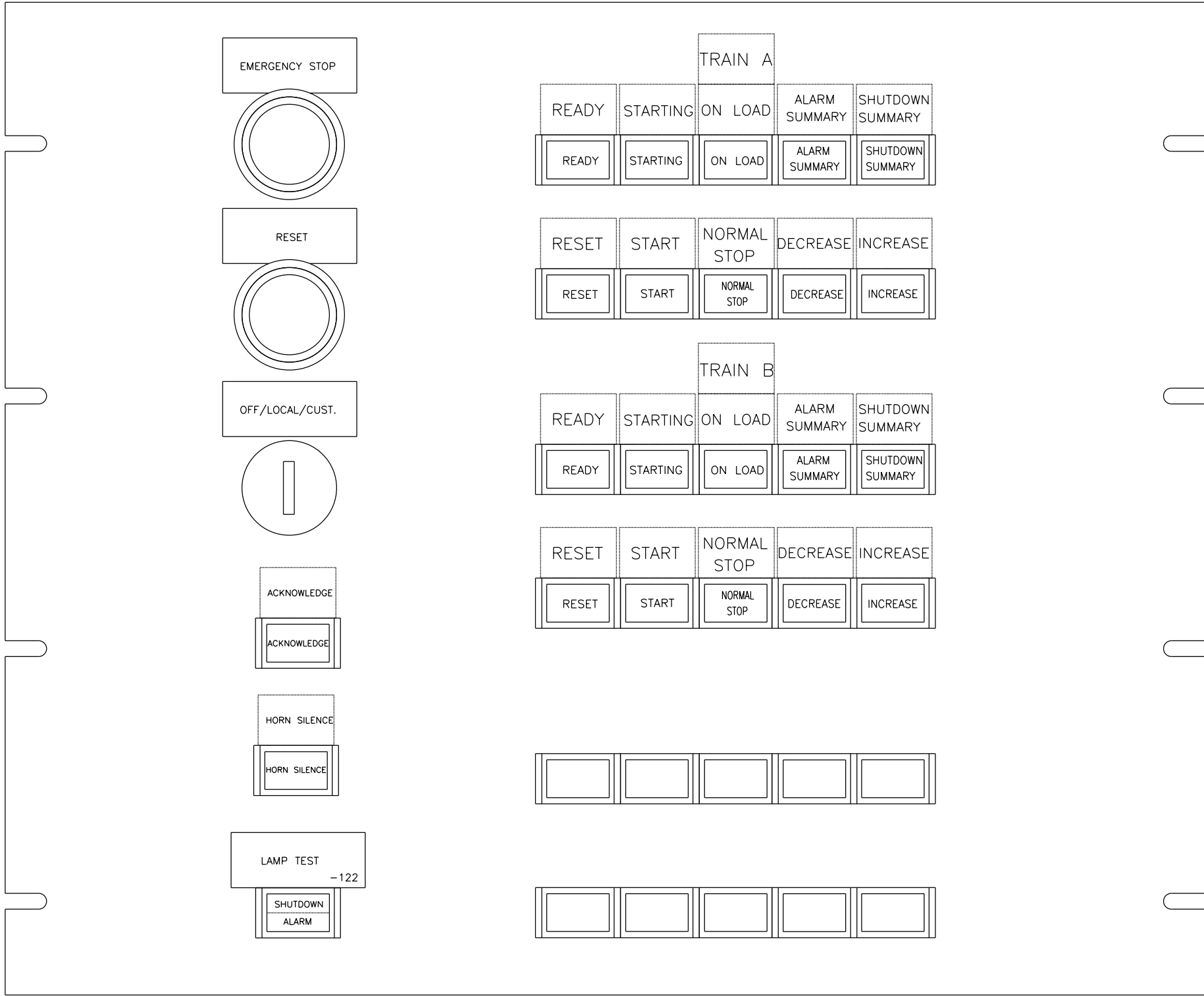
FRONT VIEW
